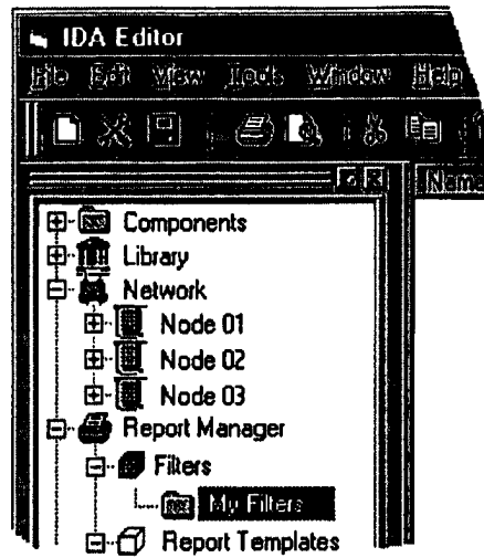
Figure 44 - Organizational Folders
